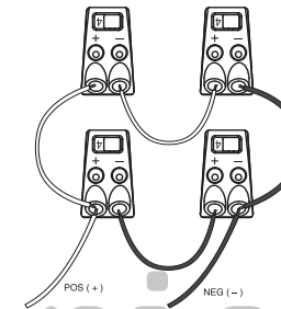
Figure 4. Four woofers connected in series-parallel
